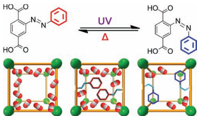
Figure 1. (Top) Trans -to- cis isomerization of the ligand of PCN-123 (PCN represents porous coordination networks) induced by UV irradiation and the cis -to- trans isomerization induced by heat treatment. (Bottom) Schematic illustration showing the suggested CO 2 uptake in MOF-5, PCN-123 trans , and PCN-123 cis .
